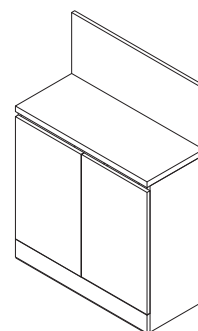
7 50822 MODULO LISCIO 80 SMOOTH MODULE 80 ↑ 1130 mm ↗ 400 mm → 800 mm
